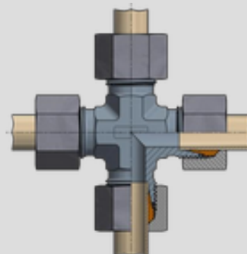
Equal Elbows, Equal Tees, Equal Crosses
