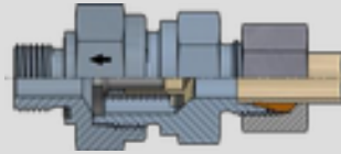
Non-Return Valves
